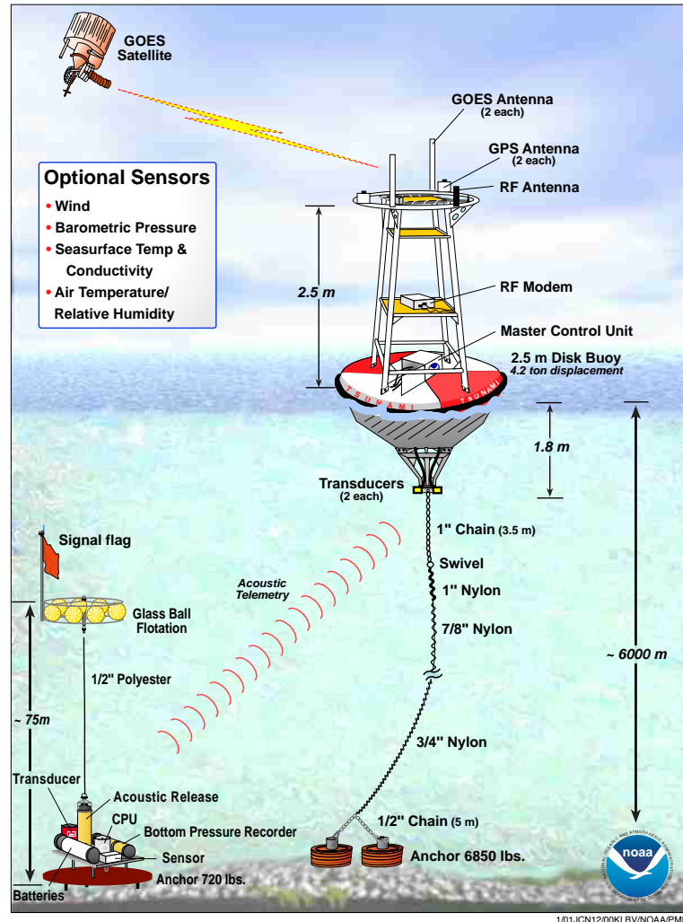
Figure 1: DART mooring system.
